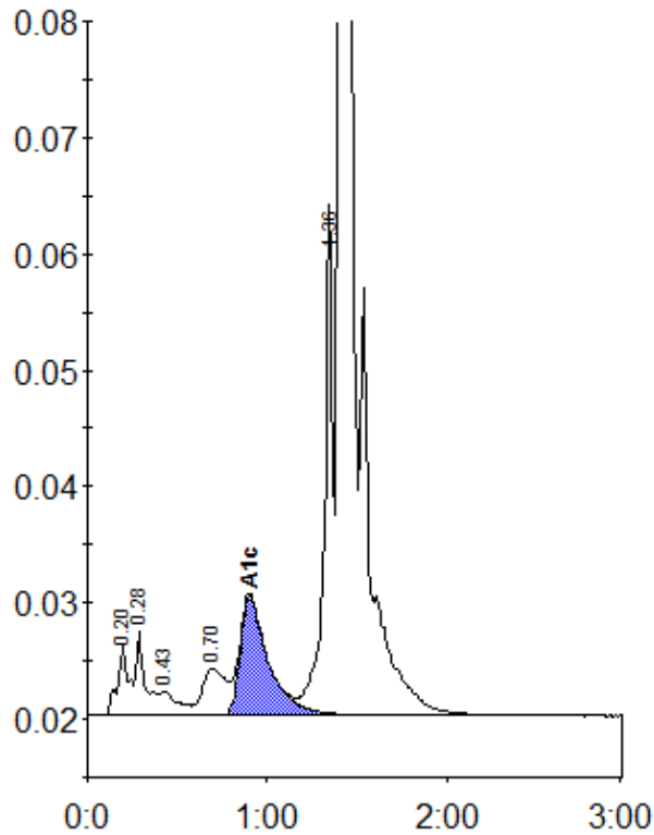
Peak table - ID: 10475035
